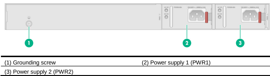
Figure 20 Rear panel
