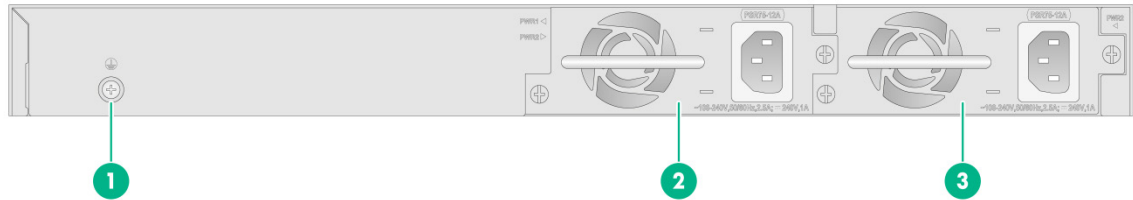
Figure 16 Rear panel
