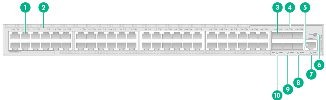
Figure 17 Front panel
