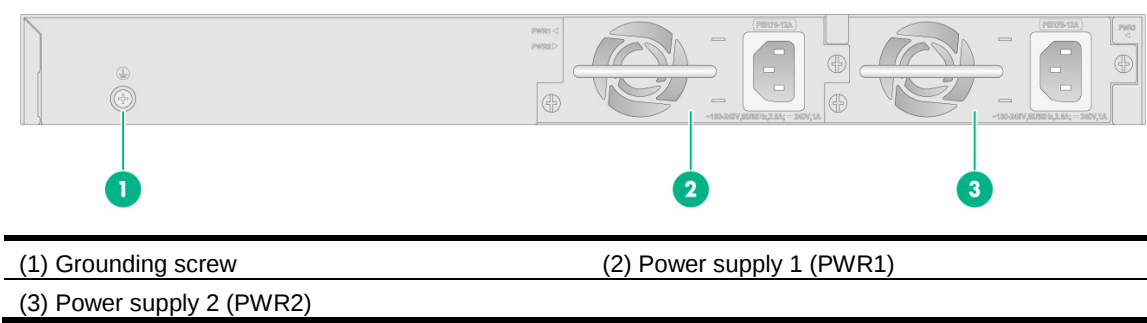
Figure 18 Rear panel
