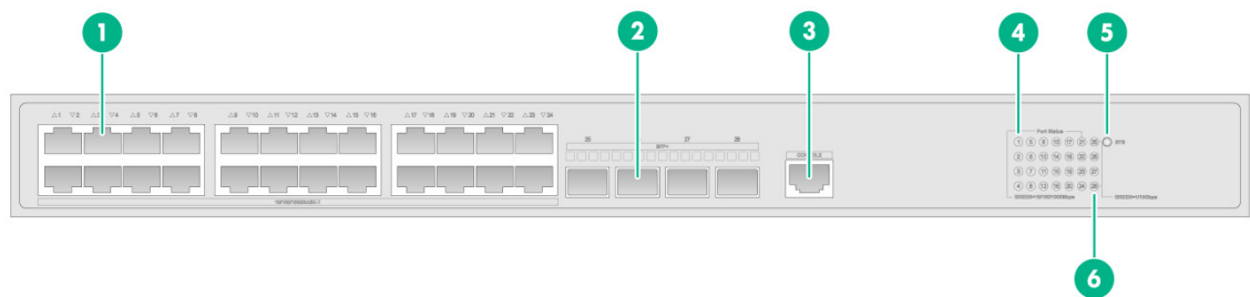
Figure 1 Front panel
