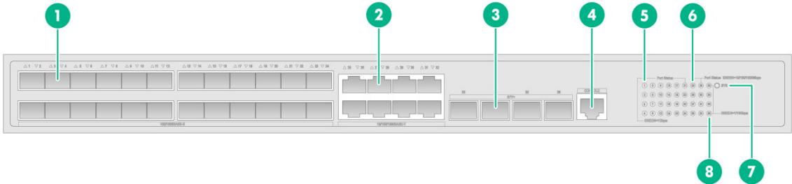
Figure 11 Front panel
