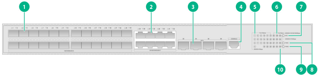
Figure 13 Front panel
