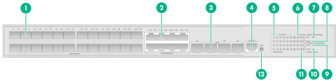
Figure 27 Front panel
